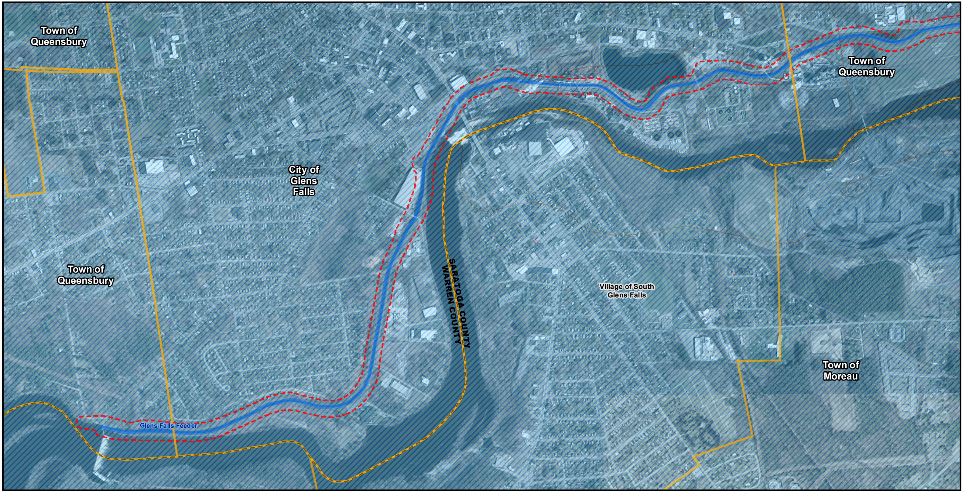
Figure 6F: Aquifers
